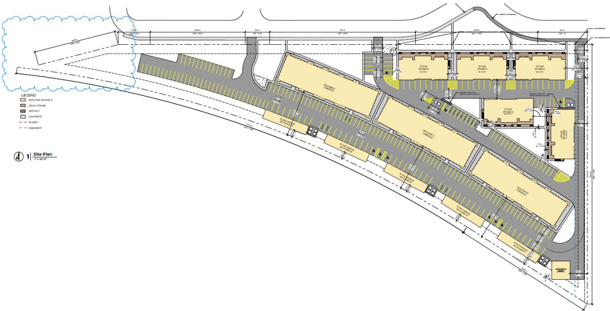
Site Plan
