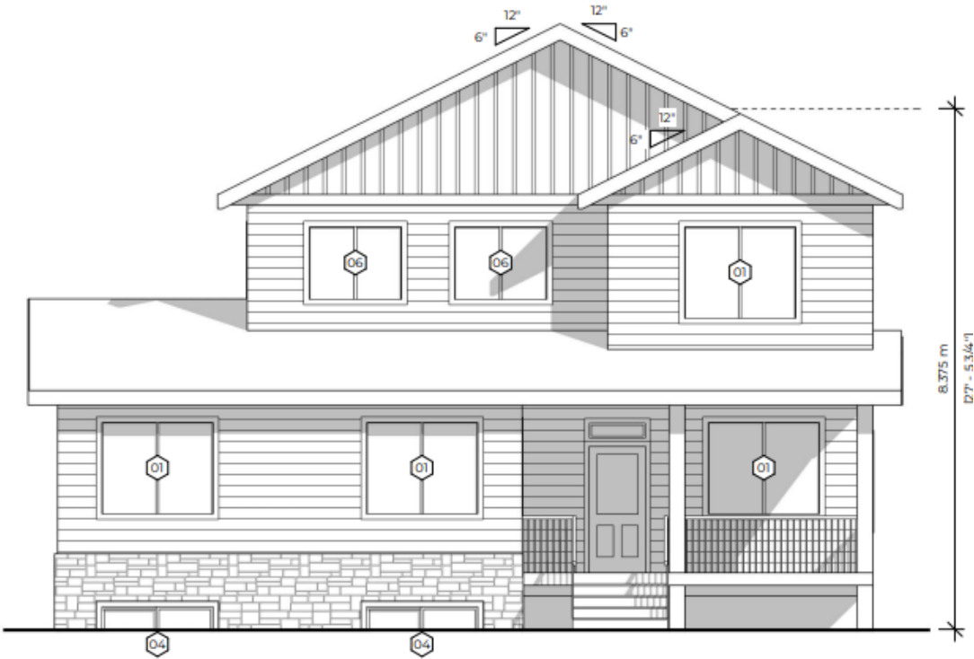
1 | Front Elevation 1/8" = 1'-0"
