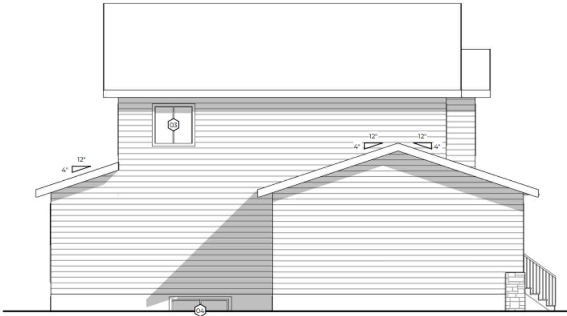
2 | Left Elevation 1/8" = 1'-0"
