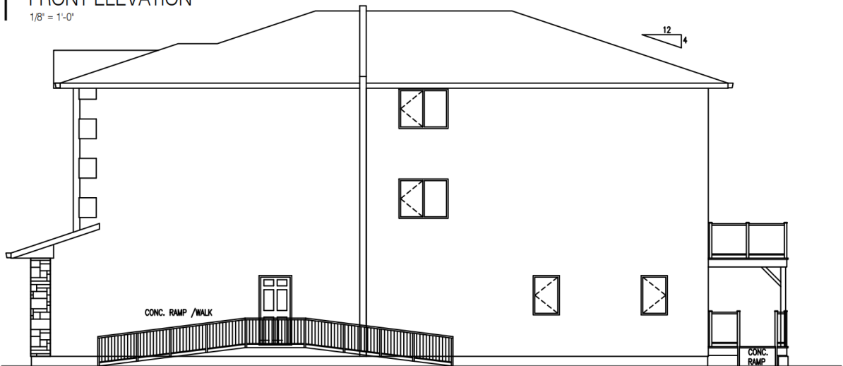
2 SIDE ELEVATION
