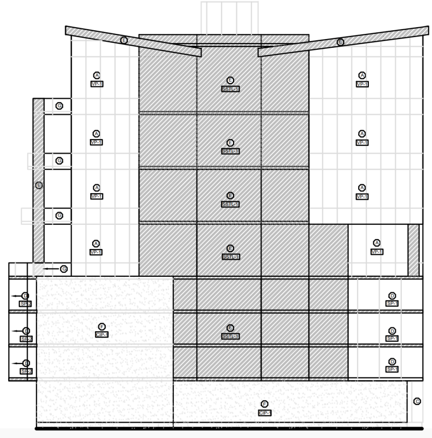
West Elevation
