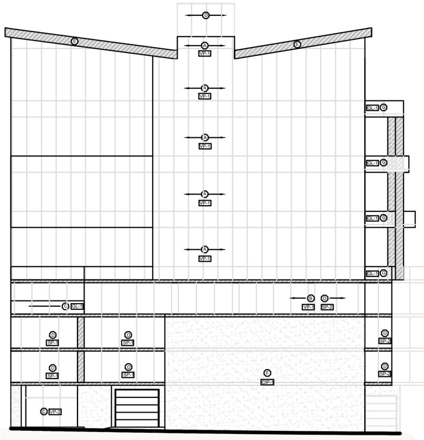
East Elevation
