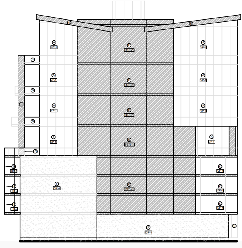
West Elevation
