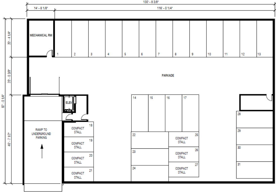
Underground Parking Plan
