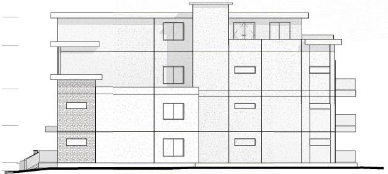
West Elevation
