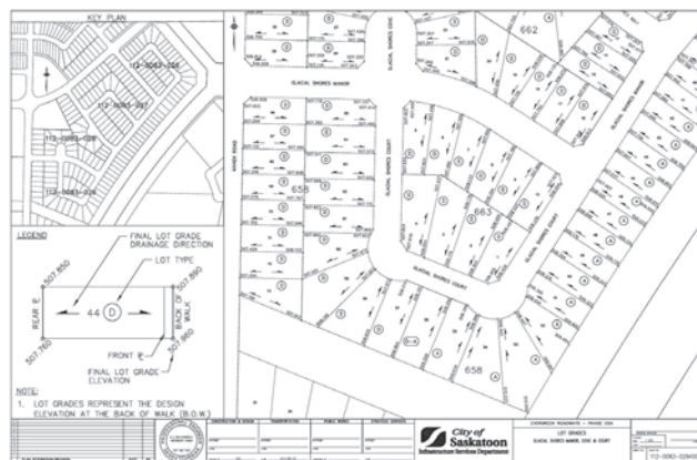
Lot Grading Plan Example
