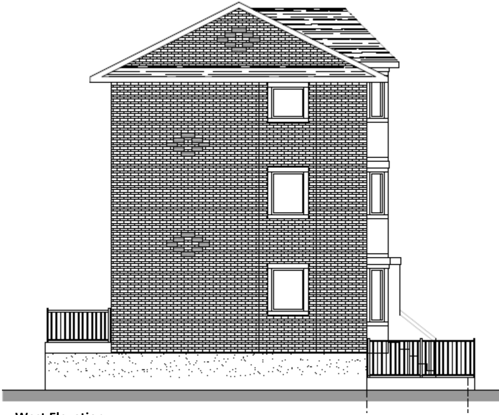
West Elevation
